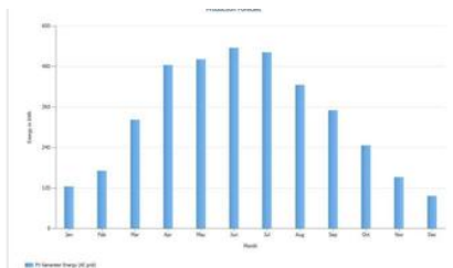
PV Generation
