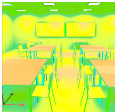
CLASSROOM CALCULATION LUX LEVELS
