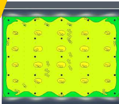
CALCULATION LUX LEVELS
